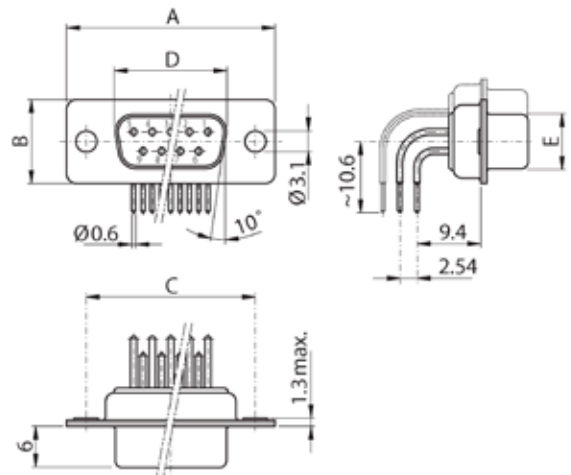
Socket connector
