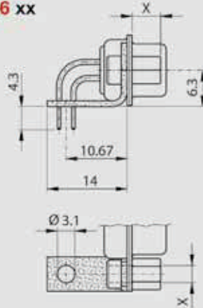
Metal Bracket
