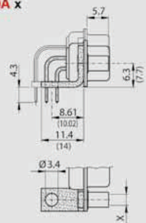
Metal Bracket
