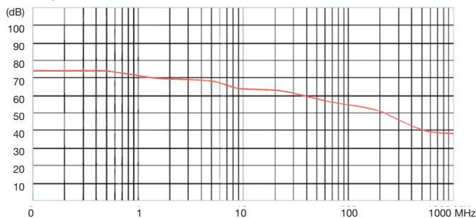
Shielding efficiency
