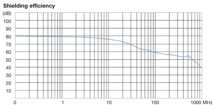
Screening Effectiveness - MHD45ZK-Series
