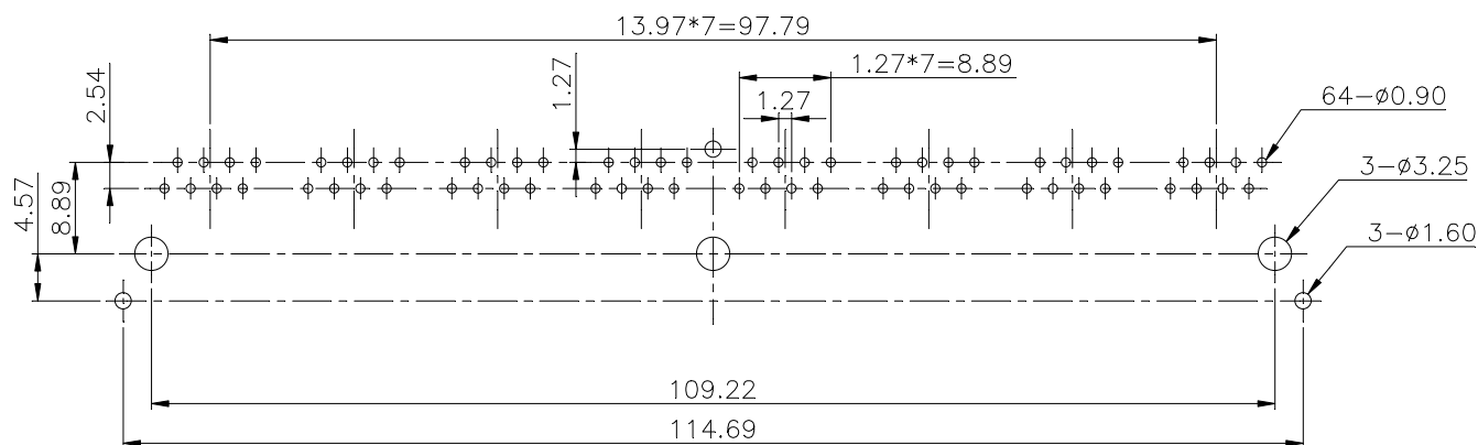
PCB LAYOUT/TOP VIEW
