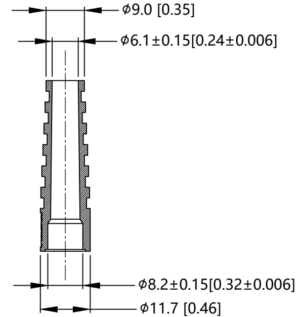
SECTION A-A (1:1)
